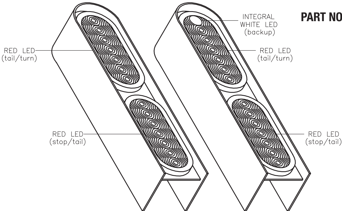
234-1 LIGHT KIT
